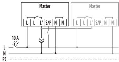
Standard operation with optional control via a closing button and parallel wiring of max. five devices.
