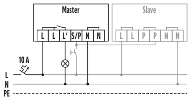
Standard operation with optional control via a closing button, and use of max. six slave devices to one master device.
