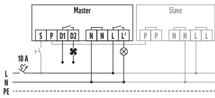
Standard operation with optional control via a closing button, and use of max. six slave devices to one master device.
