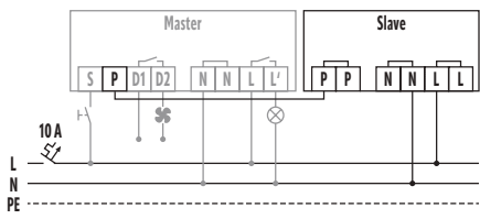
Master/slave connection for presence detectors: a maximum of 6 slave devices may be connected to one master.
