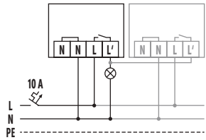
Standard operation with optional parallel wiring of max. six devices.
