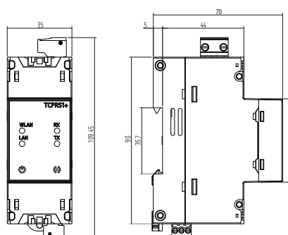
TCPRS1+
