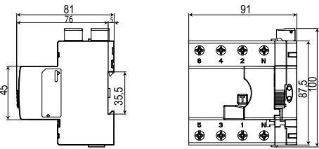
RECB-C
