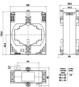
TD 10
