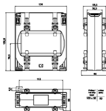
TD 12
