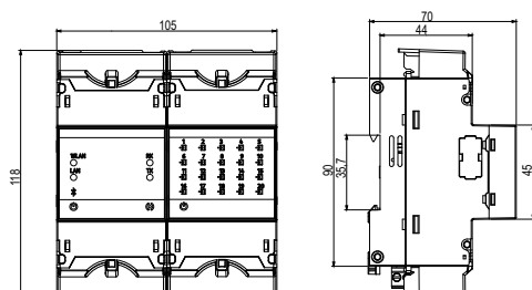
Kit Line-TCPRS1/M-20
