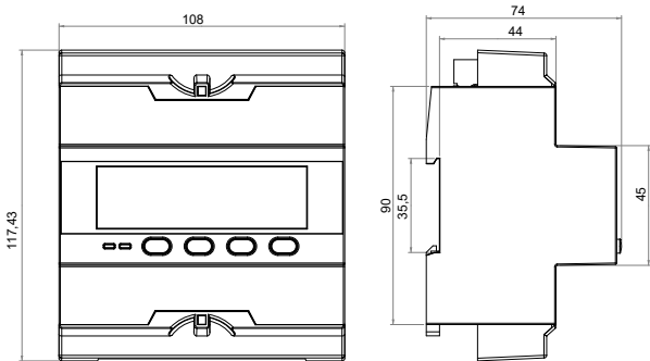
CVM-D41-DC
