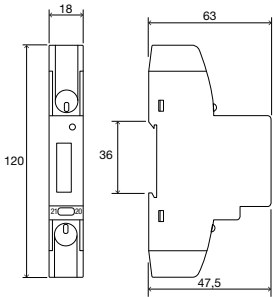
CEM-C5
