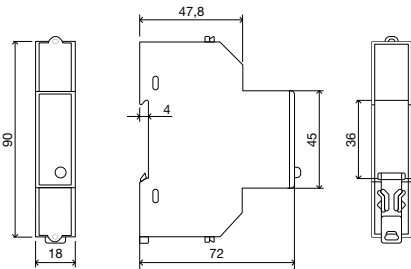
CEM-C12c
