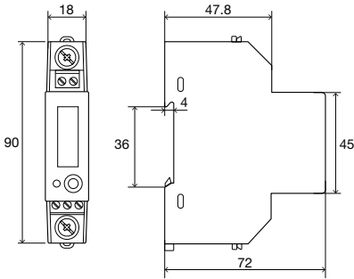
CEM-C12
