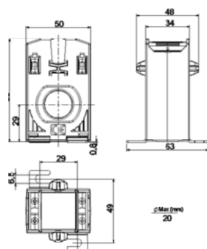
TD 4
