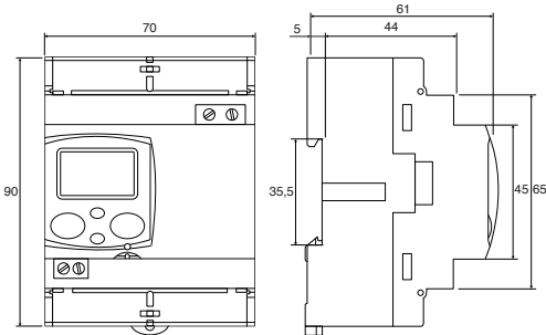
CEM-C21 / CEM-C31
