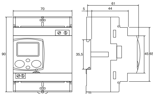
CEM-C21-485
