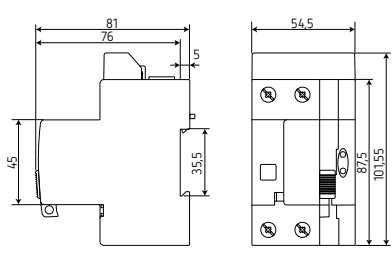
RGU-10 / CBS-4
