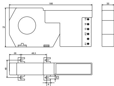
WGB-35-TB
