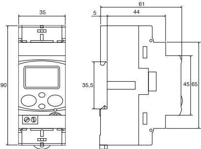
CEM-C10
