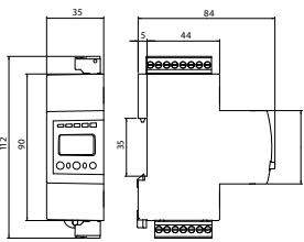
RGU2
