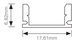
Perfil Saliente Surface Mouted Profile Profilé Surface
